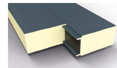
Standard lock for a wall panel GS insPIRe® S
