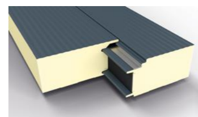
Concealed lock for GS insPIRe® U wall panel
