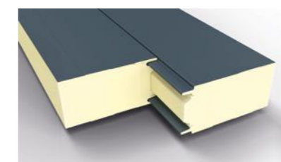
Lock for the GS insPIRe® CH cooling panel
